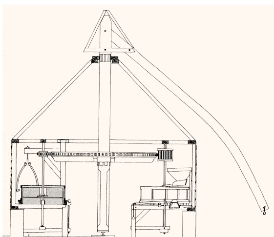
(foto 1) Rosmolen
